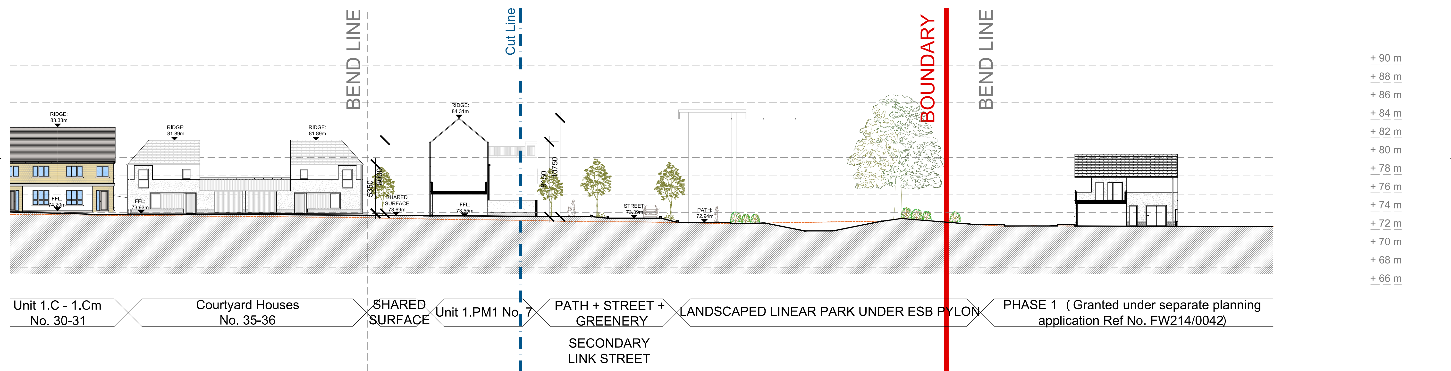
PROPOSED SITE SECTION EE (Part 2) - scale 1:200
